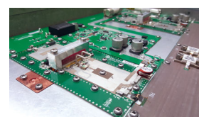
2 planar design RF pallets each of 1.25 kW
