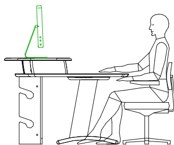
SIDE SECTION
