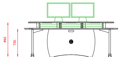
ProLite including 3 x 3U Top Racks & Monitor Bridge
